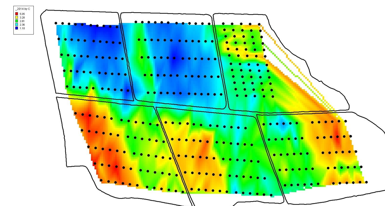
Fig. 2 Soil organic matter content (loss on ignition at 400°C)
